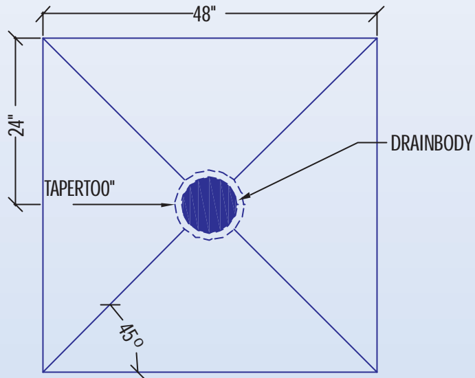
DEPICTION FOR TAPERED INSULATION
